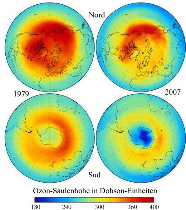
Fig. 3: The ozone layer in the Northern (Upper) and Southern (Lower)
