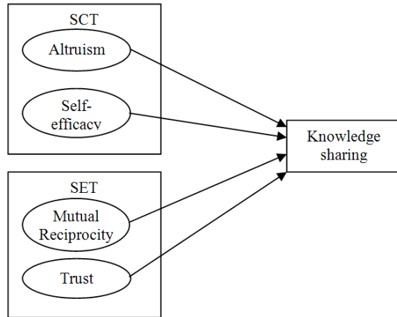
Fig. 1: Conceptual framework
